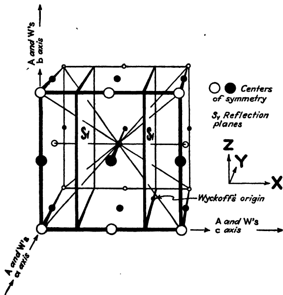
FIG. 9.—Space-group V_h^{16} .
